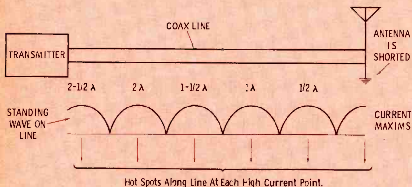
Fig. 2 Current distribution along the line is shown for a shorted condition at the antenna. Note that high density current is found at each half wave along the line, starting at the short.
