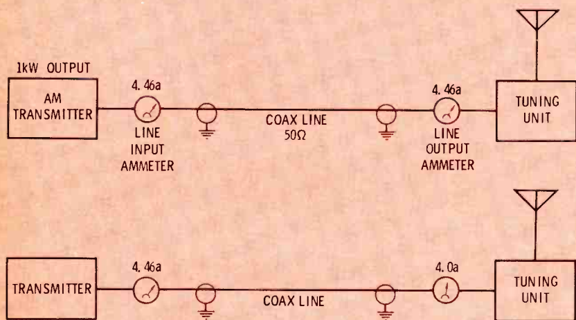
Fig. 3 Coax line on AM antenna showing balanced current at both line meters when load is properly matched to the line. Lower condition indicates incorrect match of load to line impedance.
