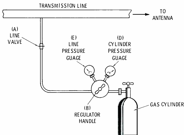
Fig. 4 Method of correctly setting line pressure regulator.
